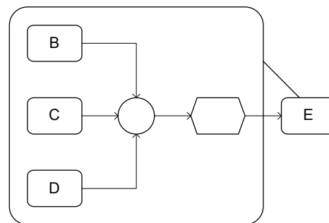
Figure 8: Workflow Patterns 9, 19-20
