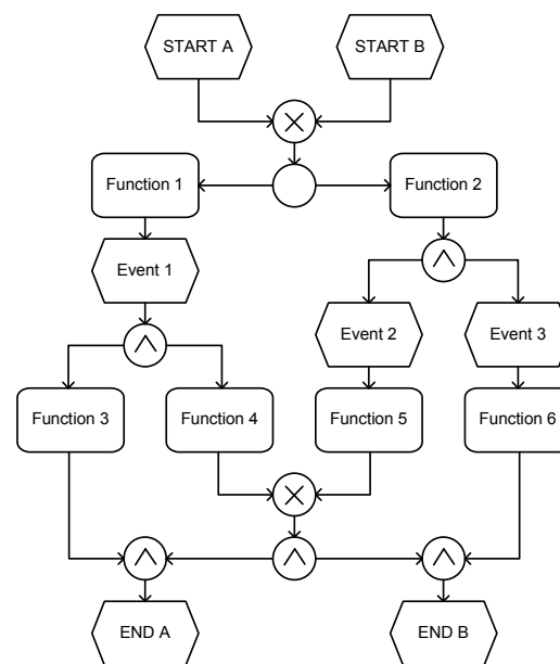
Figure 10: Example yEPC
