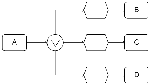
Workflow Pattern 6: Multiple Choice
