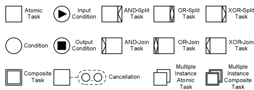
Figure 9: YAWL notation
