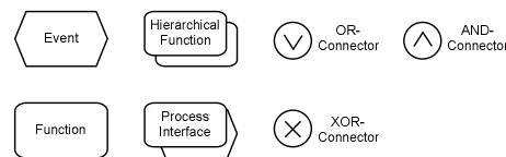
Figure 1: Symbols of the EPC notation
