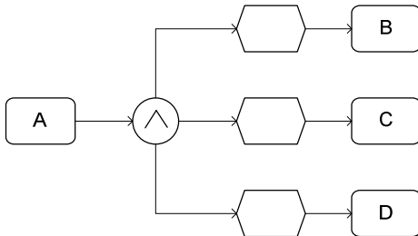
Workflow Pattern 2: Parallel Split
