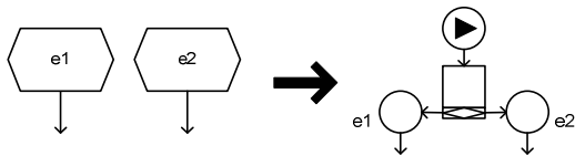
Figure 11: Mapping of Multiple Start Events
