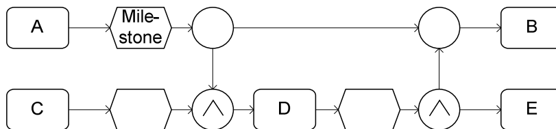
Figure 6: Workflow Patterns 17 and 18 as yEPC models
