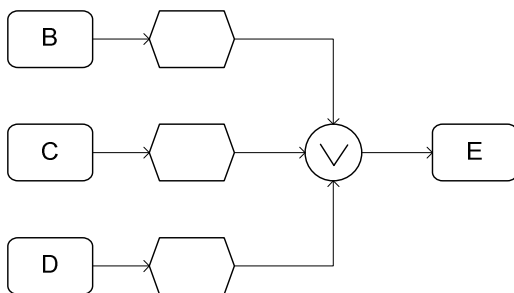
Workflow Pattern 7: Synchronizing Merge
