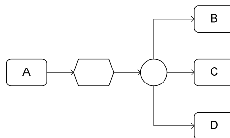
Figure 5: Workflow Patterns 8 and 16 as yEPC models
